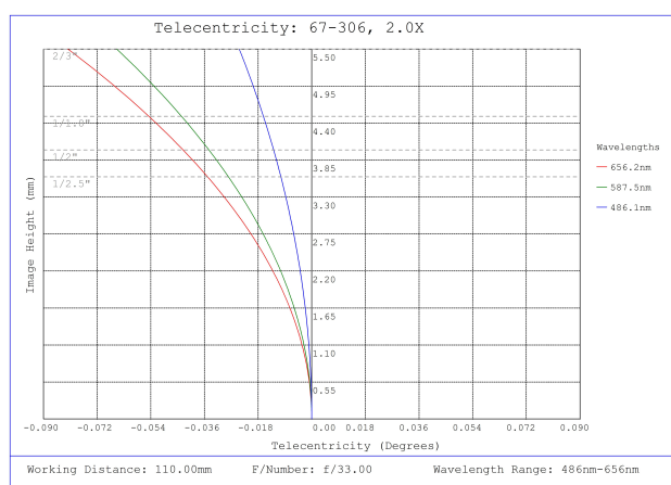
#67-306, 2X, 110mm WD, In-Line CompactTL™ Telecentric Lens, Telecentricity Plot
