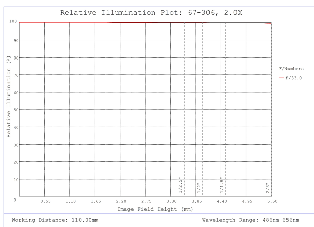
#67-306, 2X, 110mm WD, In-Line CompactTL™ Telecentric Lens, Relative Illumination Plot
