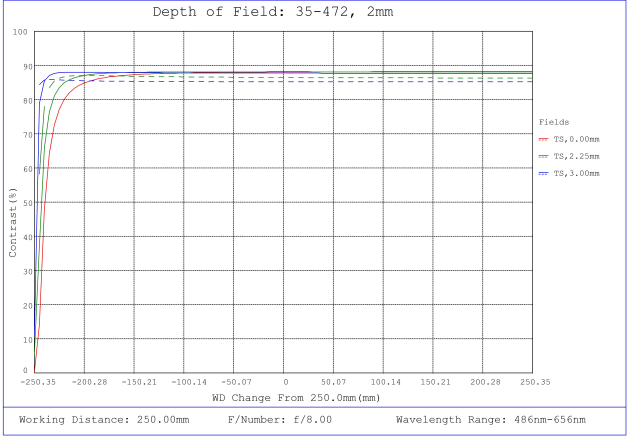
#35-472, 2mm FL f/8 IR-Cut Rugged Blue Series M12 Lens, Depth of Field Plot, 250mm Working Distance, f8
