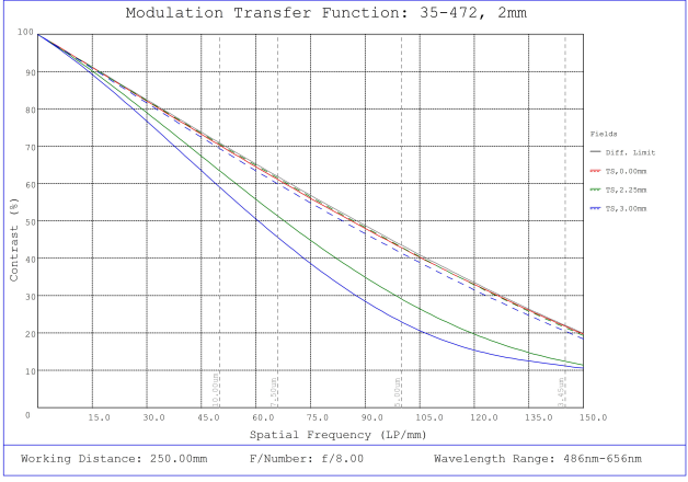
#35-472, 2mm FL f/8 IR-Cut Rugged Blue Series M12 Lens, Modulated Transfer Function (MTF) Plot, 250mm Working Distance, f8
