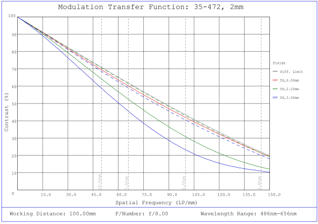
#35-472, 2mm FL f/8 IR-Cut Rugged Blue Series M12 Lens, Modulated Transfer Function (MTF) Plot, 100mm Working Distance, f8
