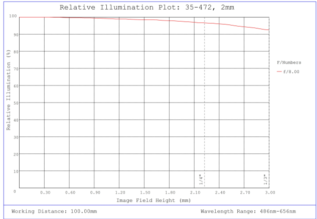
#35-472, 2mm FL f/8 IR-Cut Rugged Blue Series M12 Lens, Relative Illumination Plot
