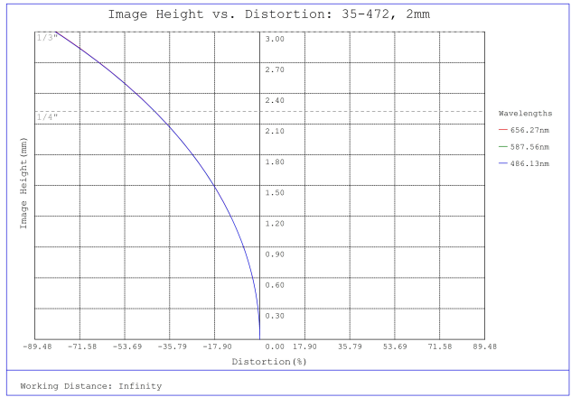
#35-472, 2mm FL f/8 IR-Cut Rugged Blue Series M12 Lens, Distortion Plot
