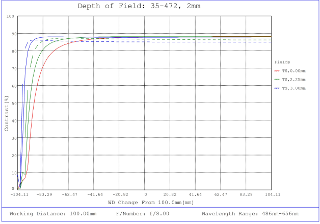
#35-472, 2mm FL f/8 IR-Cut Rugged Blue Series M12 Lens, Depth of Field Plot, 100mm Working Distance, f8
