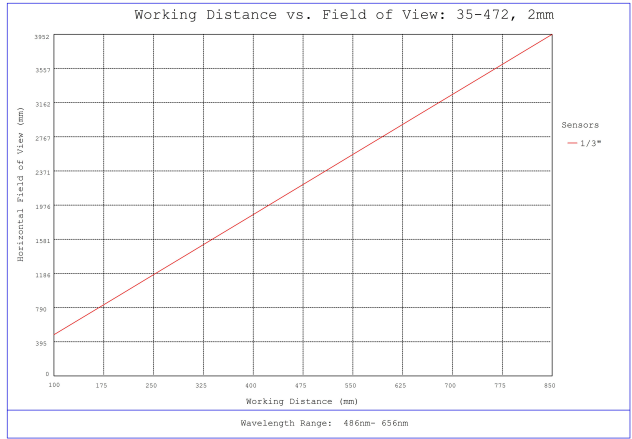
#35-472, 2mm FL f/8 IR-Cut Rugged Blue Series M12 Lens, Working Distance versus Field of View Plot
