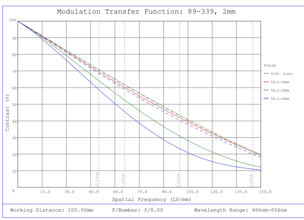
#89-339, 2mm FL f/8, Blue Series M12 Lens, Modulated Transfer Function (MTF) Plot, 100mm Working Distance, f8
