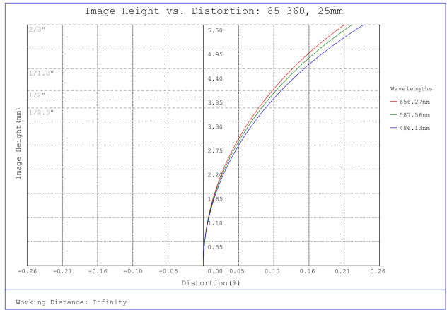
#85-360, 25mm, f/8 Ci Series Fixed Focal Length Lens, Distortion Plot
