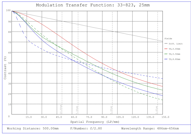
#33-823, 25mm f/2.8, HPI Series Fixed Focal Length Lens, Modulated Transfer Function (MTF) Plot, 500mm Working Distance, f2.8
