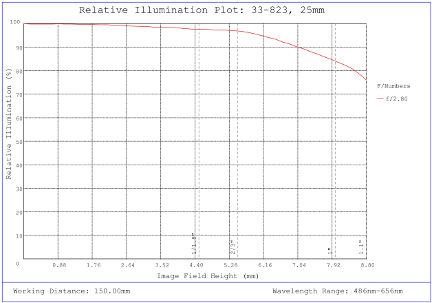
#33-823, 25mm f/2.8, HPI Series Fixed Focal Length Lens, Relative Illumination Plot
