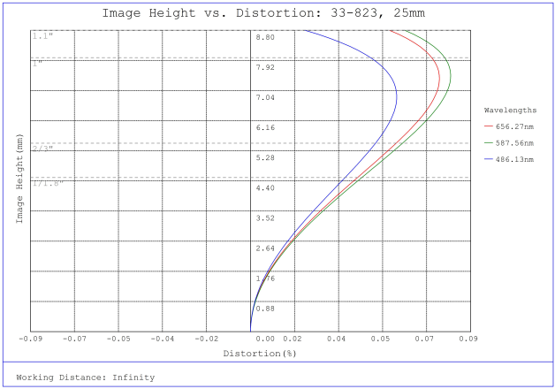
#33-823, 25mm f/2.8, HPI Series Fixed Focal Length Lens, Distortion Plot
