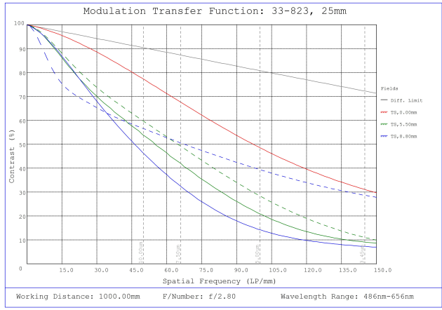
#33-823, 25mm f/2.8, HPI Series Fixed Focal Length Lens, Modulated Transfer Function (MTF) Plot, 1000mm Working Distance, f2.8
