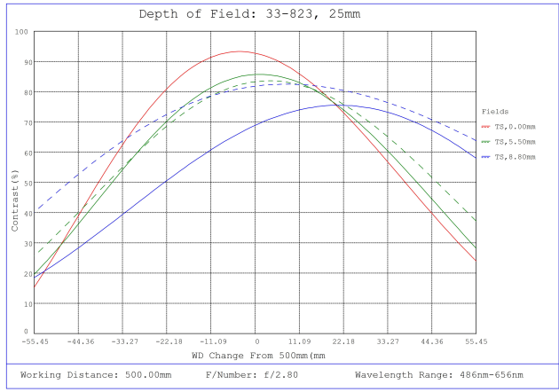
#33-823, 25mm f/2.8, HPI Series Fixed Focal Length Lens, Depth of Field Plot, 500mm Working Distance, f2.8
