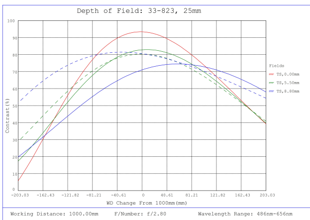
#33-823, 25mm f/2.8, HPI Series Fixed Focal Length Lens, Depth of Field Plot, 1000mm Working Distance, f2.8
