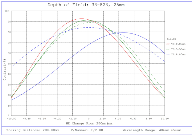
#33-823, 25mm f/2.8, HPI Series Fixed Focal Length Lens, Depth of Field Plot, 200mm Working Distance, f2.8
