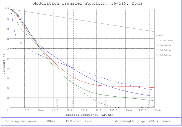
#36-519, 25mm f/2.0, HPr Series Fixed Focal Length Lens, Modulated Transfer Function (MTF) Plot, 500mm Working Distance, f2
