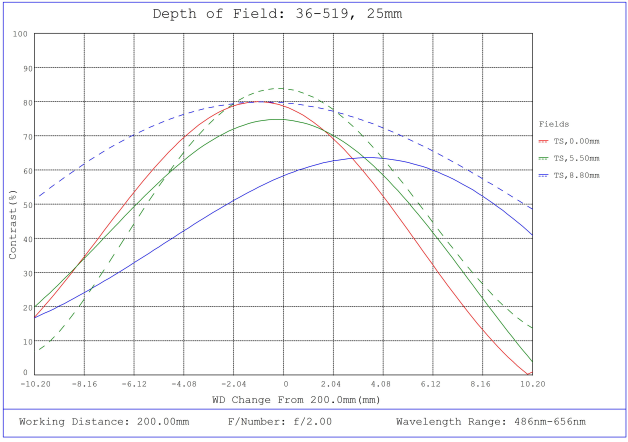
#36-519, 25mm f/2.0, HPr Series Fixed Focal Length Lens, Depth of Field Plot, 200mm Working Distance, f2
