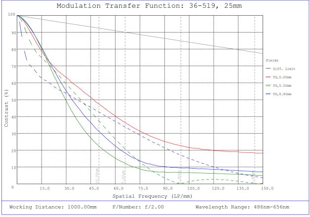
#36-519, 25mm f/2.0, HPr Series Fixed Focal Length Lens, Modulated Transfer Function (MTF) Plot, 1000mm Working Distance, f2
