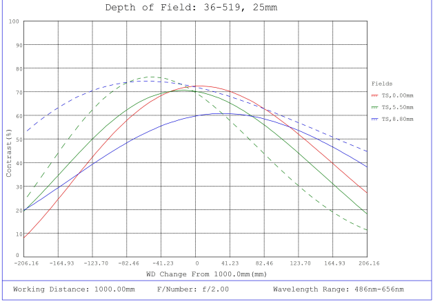
#36-519, 25mm f/2.0, HPr Series Fixed Focal Length Lens, Depth of Field Plot, 1000mm Working Distance, f2
