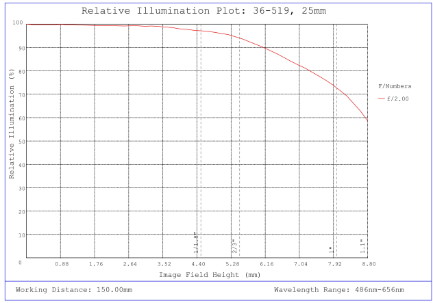
#36-519, 25mm f/2.0, HPr Series Fixed Focal Length Lens, Relative Illumination Plot
