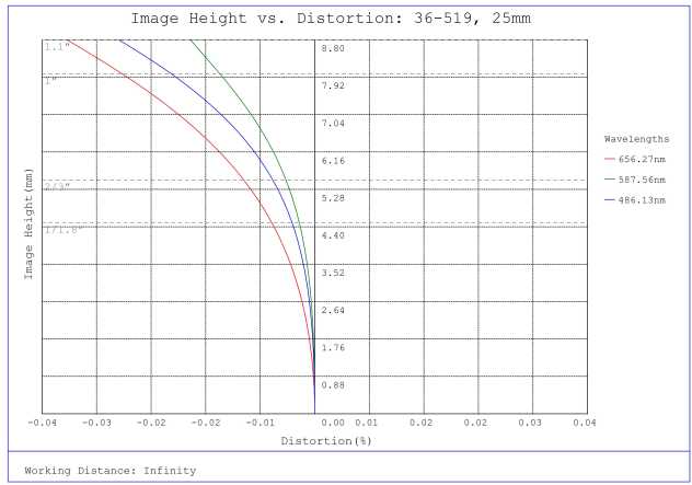
#36-519, 25mm f/2.0, HPr Series Fixed Focal Length Lens, Distortion Plot
