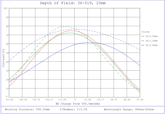
#36-519, 25mm f/2.0, HPr Series Fixed Focal Length Lens, Depth of Field Plot, 500mm Working Distance, f2
