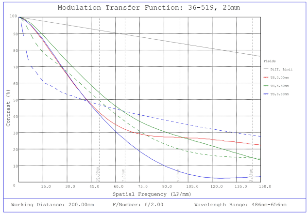
#36-519, 25mm f/2.0, HPr Series Fixed Focal Length Lens, Modulated Transfer Function (MTF) Plot, 200mm Working Distance, f2
