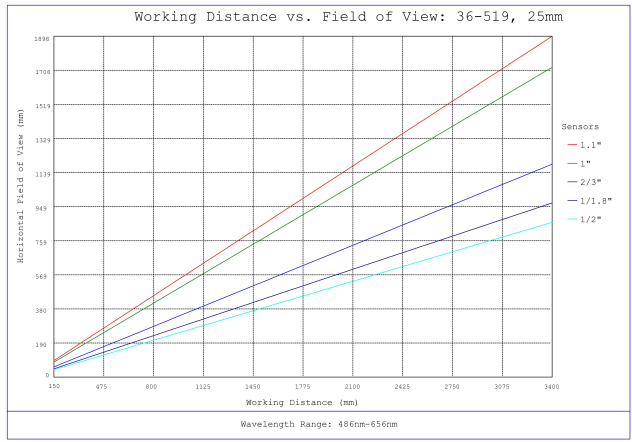
#36-519, 25mm f/2.0, HPr Series Fixed Focal Length Lens, Working Distance versus Field of View Plot
