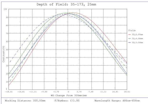
#35-173, 25mm, f/1.8 Cr Series Fixed Focal Length Lens, Depth of Field Plot, 350mm Working Distance, f1.8
