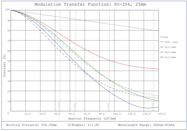
#85-356, 25mm, f/1.8 Ci Series Fixed Focal Length Lens, Modulated Transfer Function (MTF) Plot, 500mm Working Distance, f1.8
