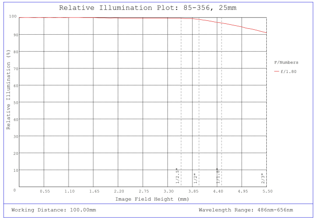
#85-356, 25mm, f/1.8 Ci Series Fixed Focal Length Lens, Relative Illumination Plot
