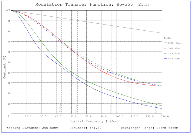
#85-356, 25mm, f/1.8 Ci Series Fixed Focal Length Lens, Modulated Transfer Function (MTF) Plot, 200mm Working Distance, f1.8
