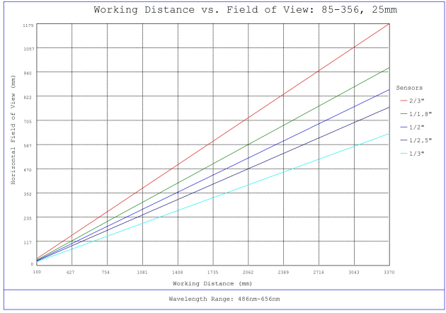
#85-356, 25mm, f/1.8 Ci Series Fixed Focal Length Lens, Working Distance versus Field of View Plot
