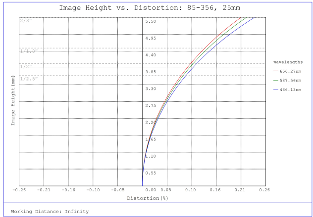
#85-356, 25mm, f/1.8 Ci Series Fixed Focal Length Lens, Distortion Plot
