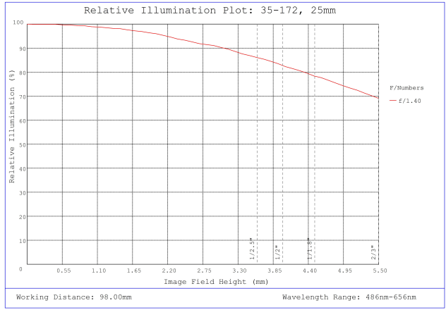
#35-172, 25mm, f/1.4 Cr Series Fixed Focal Length Lens, Relative Illumination Plot
