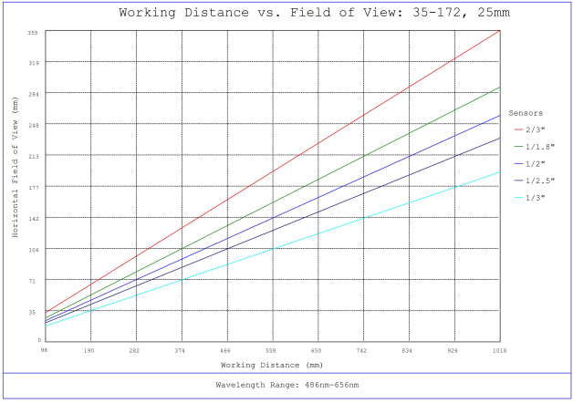
#35-172, 25mm, f/1.4 Cr Series Fixed Focal Length Lens, Working Distance versus Field of View Plot
