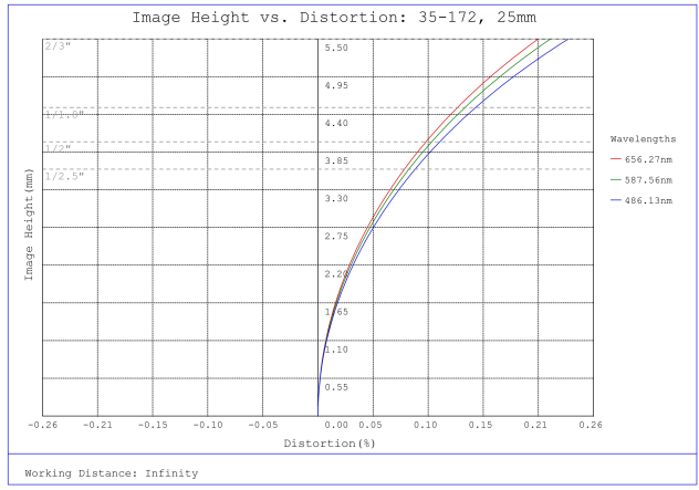
#35-172, 25mm, f/1.4 Cr Series Fixed Focal Length Lens, Distortion Plot
