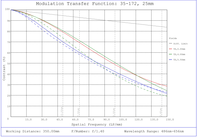
#35-172, 25mm, f/1.4 Cr Series Fixed Focal Length Lens, Modulated Transfer Function (MTF) Plot, 350mm Working Distance, f1.4
