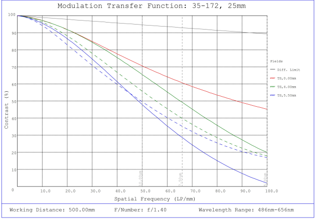
#35-172, 25mm, f/1.4 Cr Series Fixed Focal Length Lens, Modulated Transfer Function (MTF) Plot, 500mm Working Distance, f1.4
