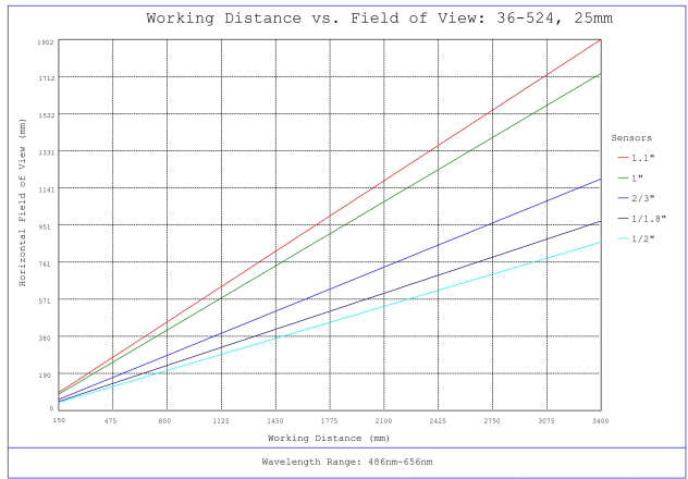
#36-524, 25mm f/11.0, HPr Series Fixed Focal Length Lens, Working Distance versus Field of View Plot
