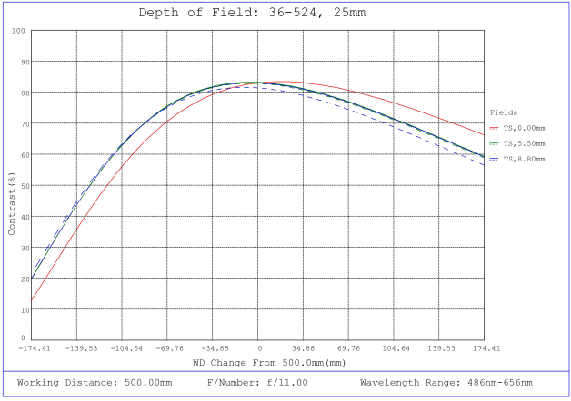
#36-524, 25mm f/11.0, HPr Series Fixed Focal Length Lens, Depth of Field Plot, 500mm Working Distance, f11
