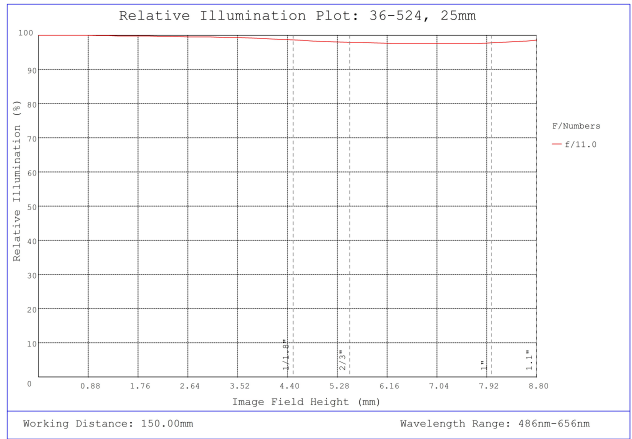
#36-524, 25mm f/11.0, HPr Series Fixed Focal Length Lens, Relative Illumination Plot
