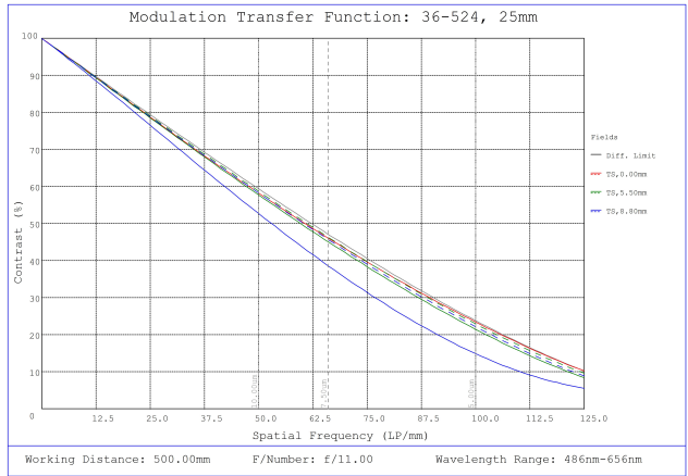
#36-524, 25mm f/11.0, HPr Series Fixed Focal Length Lens, Modulated Transfer Function (MTF) Plot, 500mm Working Distance, f11
