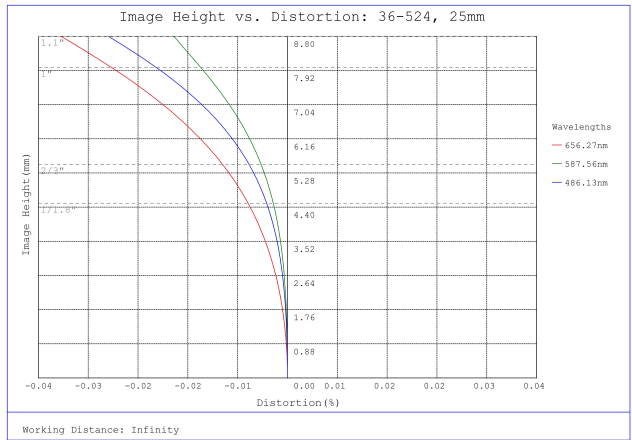
#36-524, 25mm f/11.0, HPr Series Fixed Focal Length Lens, Distortion Plot
