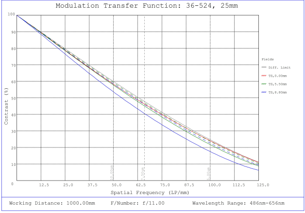
#36-524, 25mm f/11.0, HPr Series Fixed Focal Length Lens, Modulated Transfer Function (MTF) Plot, 1000mm Working Distance, f11
