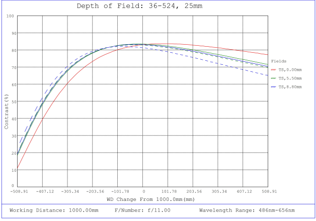
#36-524, 25mm f/11.0, HPr Series Fixed Focal Length Lens, Depth of Field Plot, 1000mm Working Distance, f11
