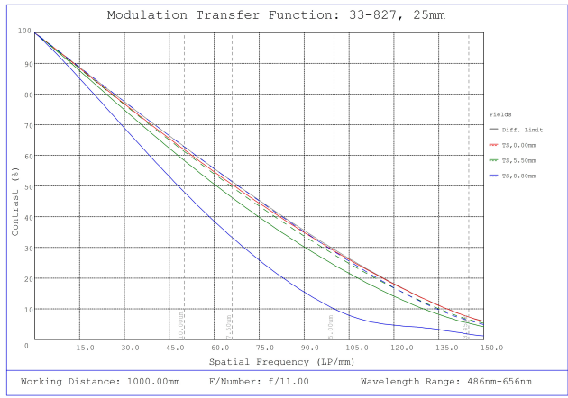
#33-827, 25mm f/11.0, HPi Series Fixed Focal Length Lens, Modulated Transfer Function (MTF) Plot, 1000mm Working Distance, f11
