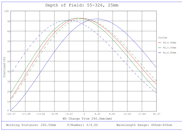
#55-326, 25mm DG Series Fixed Focal Length Lens, Depth of Field Plot, 240mm Working Distance, f4
