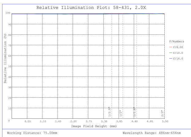
#58-431, 2.0X SilverTL™ Telecentric Lens, Relative Illumination Plot
