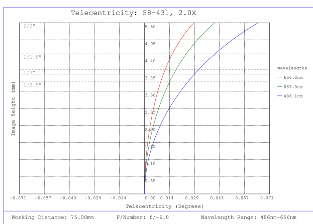
#58-431, 2.0X SilverTL™ Telecentric Lens, Telecentricity Plot
