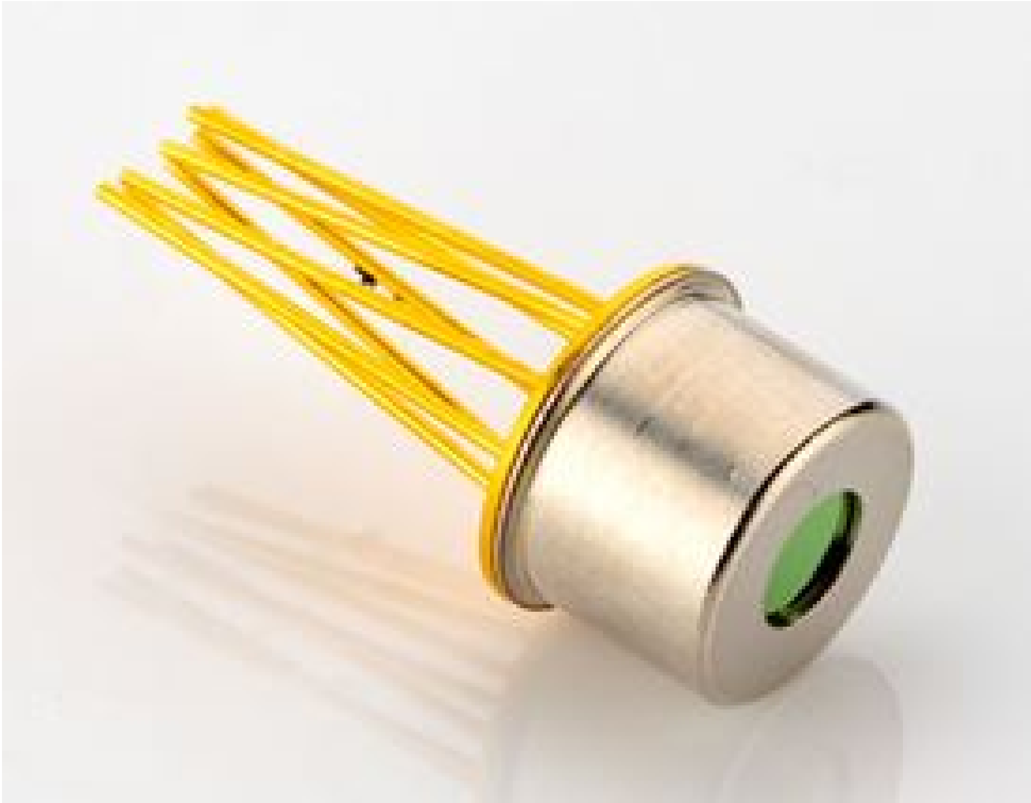
2 - 5.5um InAsSb Photovoltaic Multi-Junction IR Detector, PVMA-1TE-5-1x1-TO39-pSiAR-70
