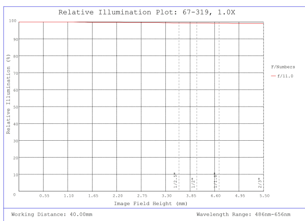
#67-319, 1X, 40mm WD, In-Line CompactTL™ Telecentric Lens, Relative Illumination Plot
