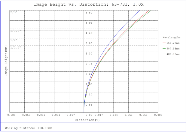
#63-731, 1X, 110mm WD CompactTL™ Telecentric Lens, Distortion Plot
