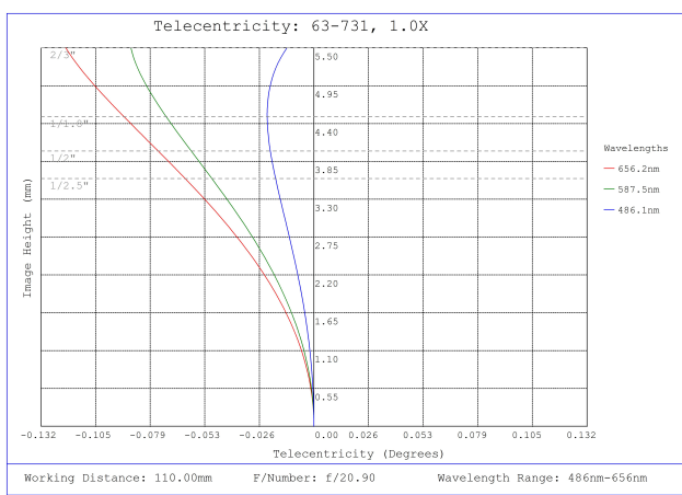
#63-731, 1X, 110mm WD CompactTL™ Telecentric Lens, Telecentricity Plot
