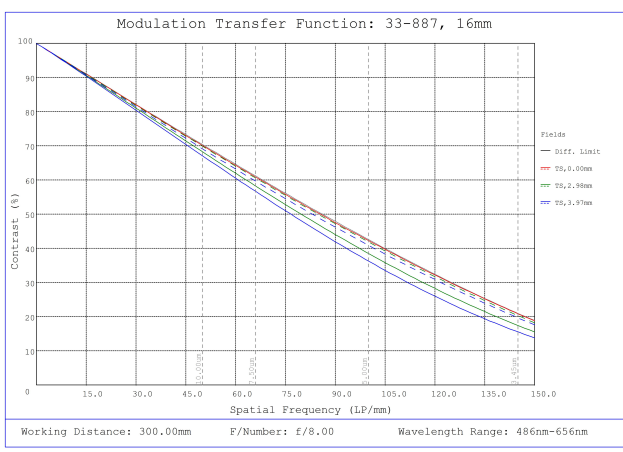
#33-887, 16mm, f/8 UCI Series Fixed Focal Length Lens, Modulated Transfer Function (MTF) Plot, 300mm Working Distance, f8
