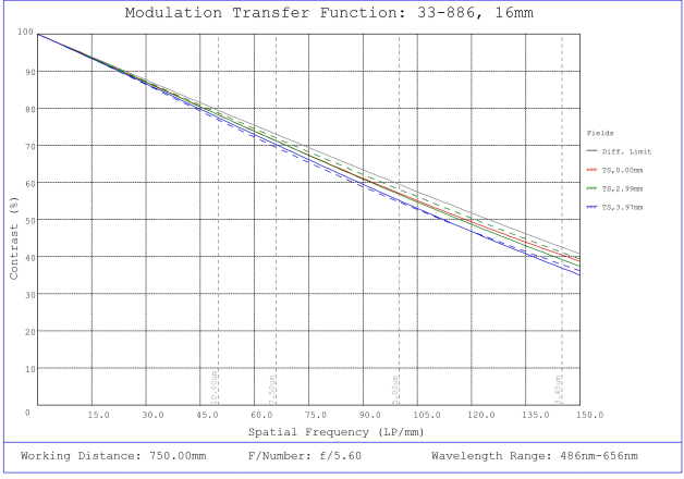
#33-886, 16mm, f/5.6 UCI Series Fixed Focal Length Lens, Modulated Transfer Function (MTF) Plot, 750mm Working Distance, f5.6
