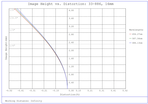
#33-886, 16mm, f/5.6 UCi Series Fixed Focal Length Lens, Distortion Plot
