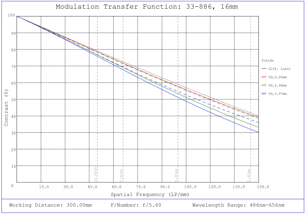
#33-886, 16mm, f/5.6 UCI Series Fixed Focal Length Lens, Modulated Transfer Function (MTF) Plot, 300mm Working Distance, f5.6
