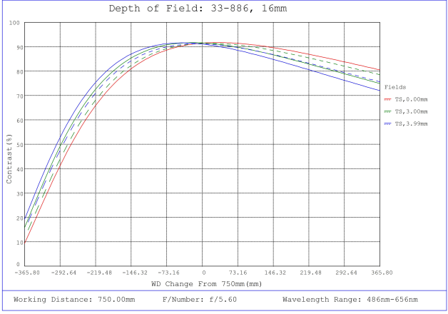
#33-886, 16mm, f/5.6 UCI Series Fixed Focal Length Lens, Depth of Field Plot, 750mm Working Distance, f5.6
