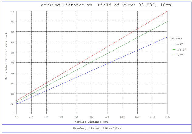
#33-886, 16mm, f/5.6 UCi Series Fixed Focal Length Lens, Working Distance versus Field of View Plot
