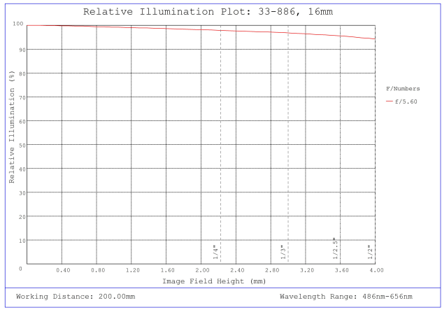
#33-886, 16mm, f/5.6 UCi Series Fixed Focal Length Lens, Relative Illumination Plot
