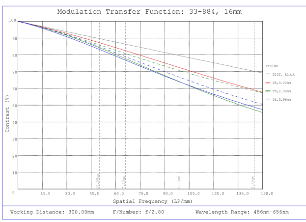
#33-884, 16mm, f/2.8 UCI Series Fixed Focal Length Lens, Modulated Transfer Function (MTF) Plot, 300mm Working Distance, f2.8
