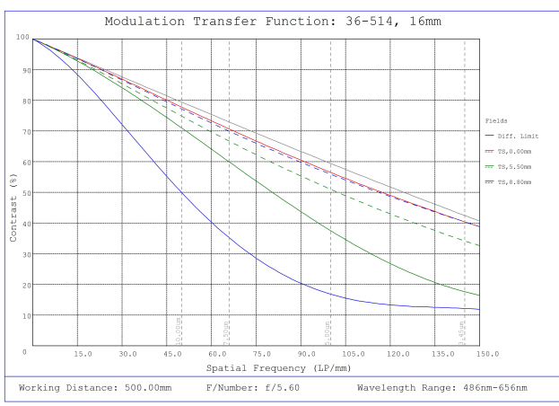
#36-514, 16mm f/5.6, HPr Series Fixed Focal Length Lens, Modulated Transfer Function (MTF) Plot, 500mm Working Distance, f5.6
