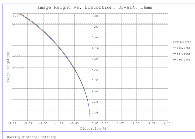
#33-814, 16mm f/1.8, HPi Series Fixed Focal Length Lens, Distortion Plot
