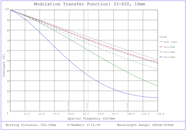
#33-820, 16mm f/16, HPi Series Fixed Focal Length Lens, Modulated Transfer Function (MTF) Plot, 500mm Working Distance, f16
