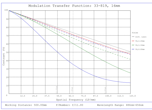
#33-819, 16mm f/11, HPI Series Fixed Focal Length Lens, Modulated Transfer Function (MTF) Plot, 500mm Working Distance, f11
