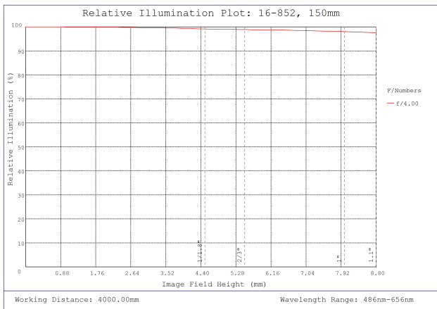
#16-852, 150mm, f/4 Athermal Lens, Relative Illumination Plot
