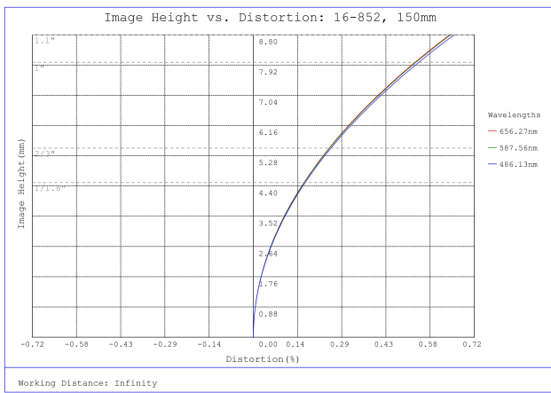
#16-852, 150mm, f/4 Athermal Lens, Distortion Plot
