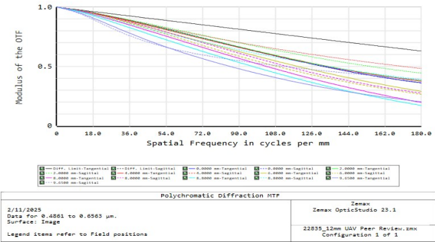
#22-835 - 12mm Focal Length, UAV Series Fixed Focal Length Lens, Modulated Transfer Function (MTF) Plot, Infinity Working Distance, f2.8
