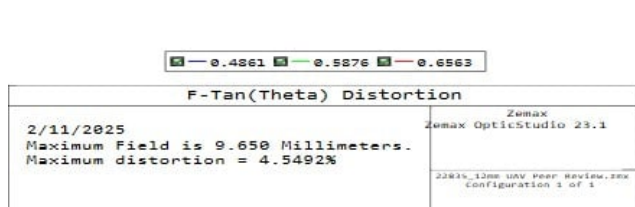
#22-835 - 12mm Focal Length, UAV Series Fixed Focal Length Lens, Distortion Plot
