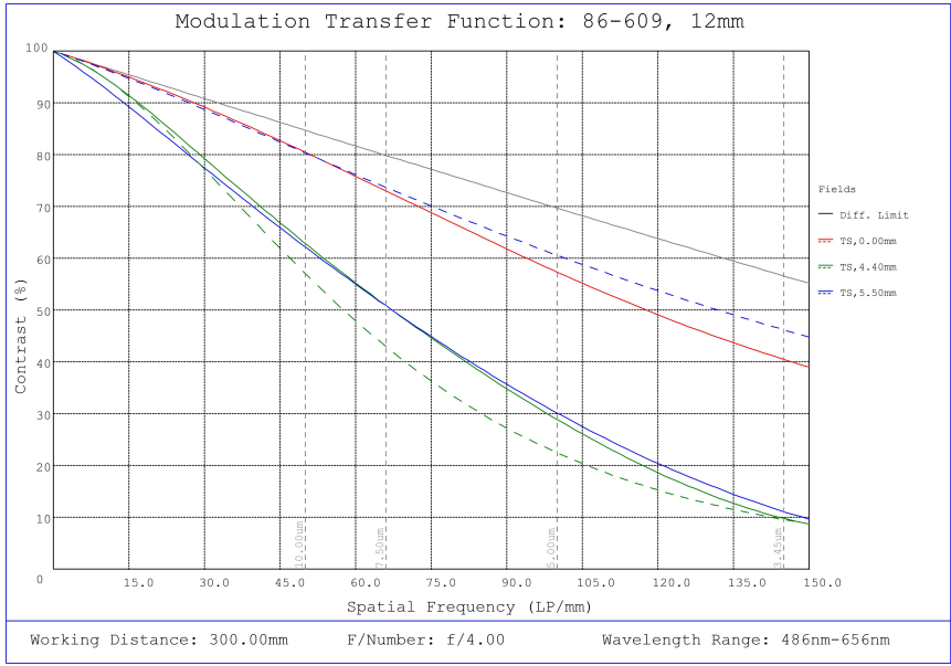
#86-609, 12mm, f/4 Ci Series Fixed Focal Length Lens, Modulated Transfer Function (MTF) Plot, 300mm Working Distance, f4
