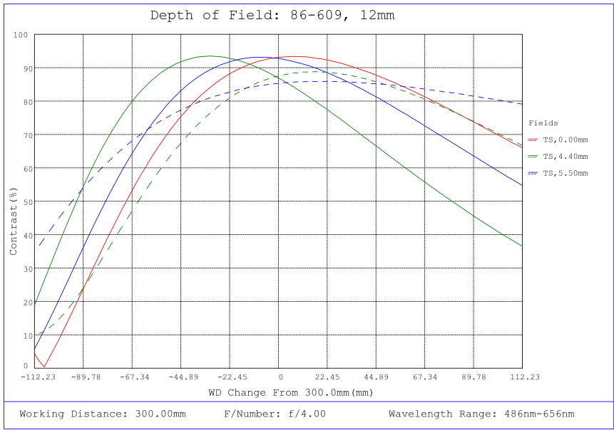
#86-609, 12mm, f/4 Ci Series Fixed Focal Length Lens, Depth of Field Plot, 300mm Working Distance, f4
