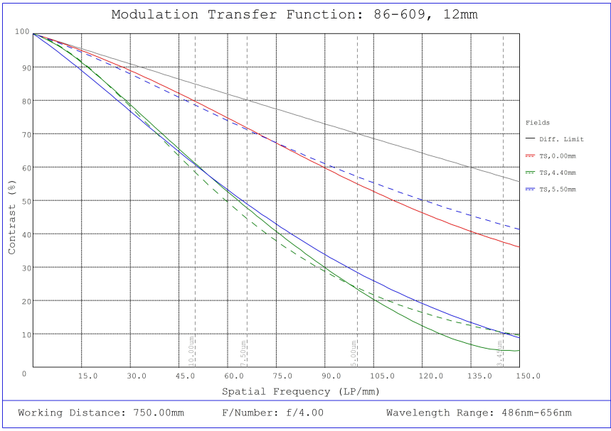
#86-609, 12mm, f/4 Ci Series Fixed Focal Length Lens, Modulated Transfer Function (MTF) Plot, 750mm Working Distance, f4
