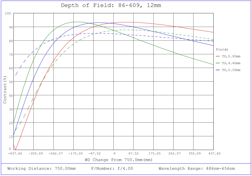
#86-609, 12mm, f/4 Ci Series Fixed Focal Length Lens, Depth of Field Plot, 750mm Working Distance, f4
