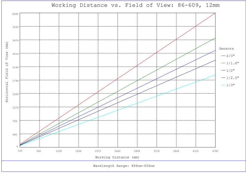
#86-609, 12mm, f/4 Ci Series Fixed Focal Length Lens, Working Distance versus Field of View Plot
