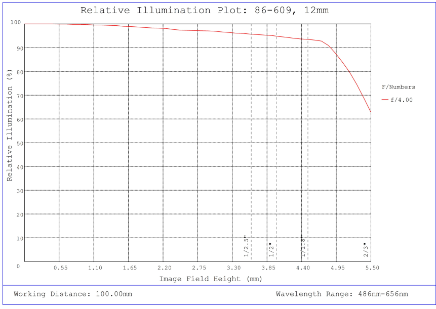
#86-609, 12mm, f/4 Ci Series Fixed Focal Length Lens, Relative Illumination Plot
