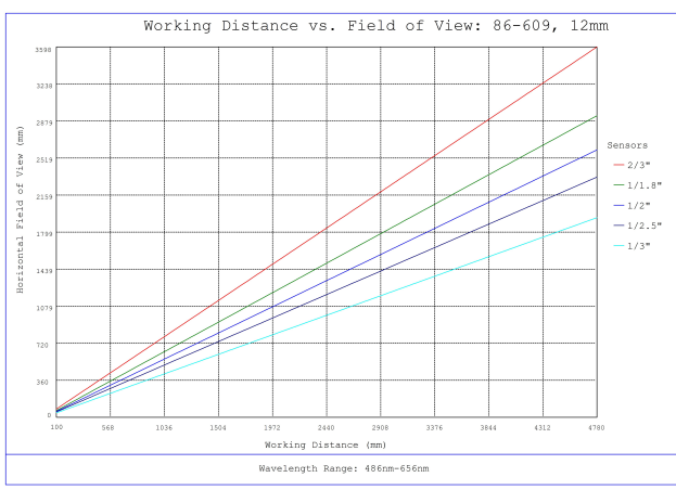
#86-609, 12mm, f/4 Ci Series Fixed Focal Length Lens, Working Distance versus Field of View Plot
