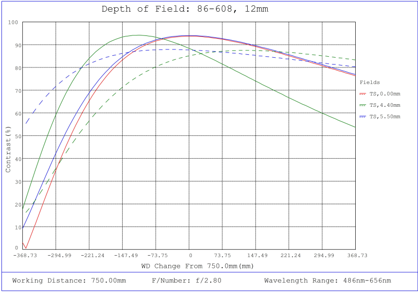
#86-608, 12mm, f/2.8 Ci Series Fixed Focal Length Lens, Depth of Field Plot, 750mm Working Distance, f2.8
