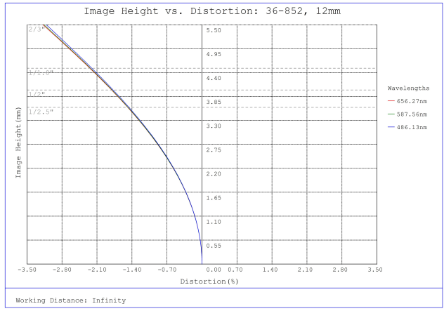
#36-852, 12mm f/4, 150-500mm Primary WD, HRr Series Fixed Focal Length Lens, Distortion Plot
