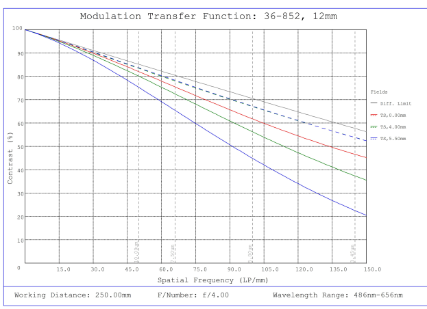
#36-852, 12mm f/4, 150-500mm Primary WD, HRr Series Fixed Focal Length Lens, Modulated Transfer Function (MTF) Plot, 250mm Working Distance, f4
