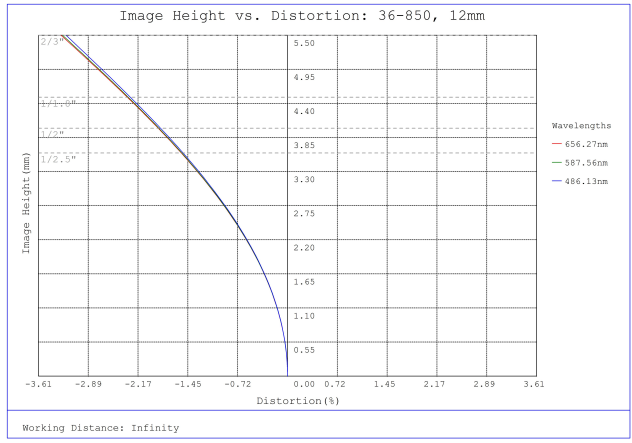
#36-850, 12mm f/2.8, 400-2000mm Primary WD, HRr Series Fixed Focal Length Lens, Distortion Plot
