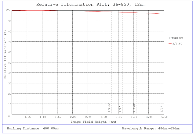
#36-850, 12mm f/2.8, 400-2000mm Primary WD, HRr Series Fixed Focal Length Lens, Relative Illumination Plot
