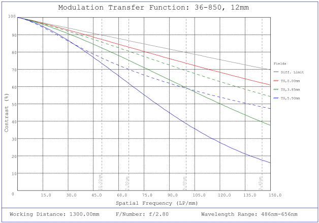
#36-850, 12mm f/2.8, 400-2000mm Primary WD, HRr Series Fixed Focal Length Lens, Modulated Transfer Function (MTF) Plot, 1300mm Working Distance, f2.8
