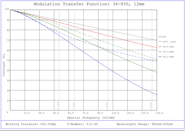
#36-850, 12mm f/2.8, 400-2000mm Primary WD, HRr Series Fixed Focal Length Lens, Modulated Transfer Function (MTF) Plot, 650mm Working Distance, f2.8
