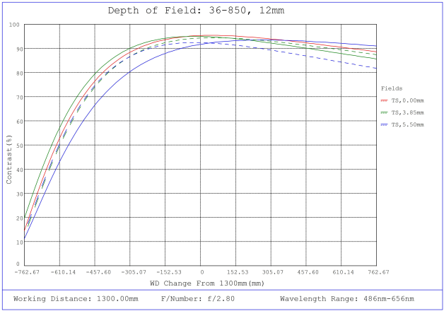
#36-850, 12mm f/2.8, 400-2000mm Primary WD, HRr Series Fixed Focal Length Lens, Depth of Field Plot, 1300mm Working Distance, f2.8
