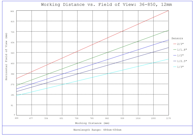
#36-850, 12mm f/2.8, 400-2000mm Primary WD, HRr Series Fixed Focal Length Lens, Working Distance versus Field of View Plot
