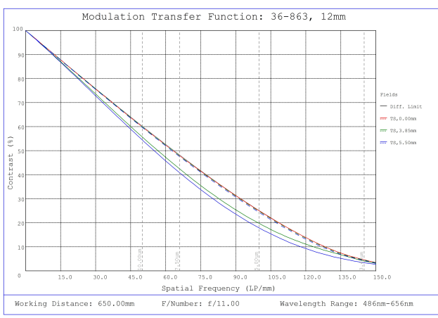
#36-863, 12mm f/11, 400-2000mm Primary WD, HRr Series Fixed Focal Length Lens, Modulated Transfer Function (MTF) Plot, 650mm Working Distance, f11
