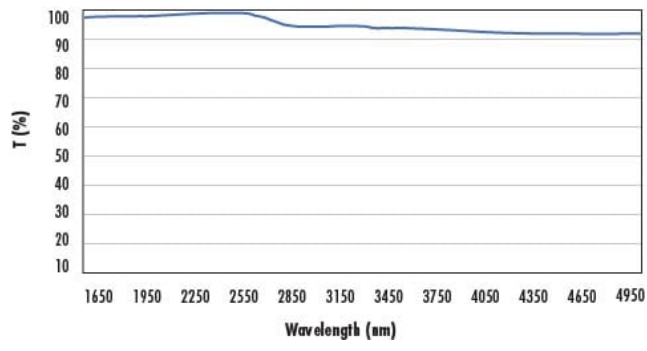
Calcium Fluoride with 2000-5000nm BBR Coating Typical Transmission
