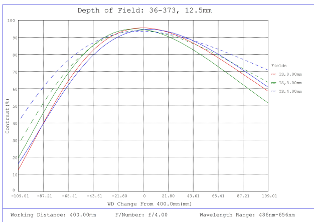
#36-373, 12.5mm FL f/4, Rugged Blue Series M12 Lens, Depth of Field Plot, 400mm Working Distance, f4
