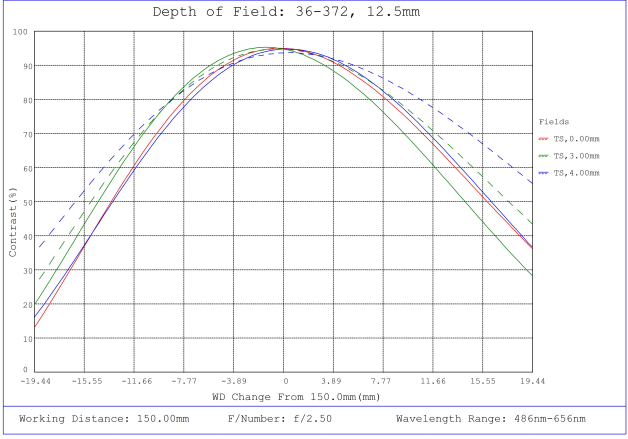
#36-372, 12.5mm FL f/2.5, Rugged Blue Series M12 Lens, Depth of Field Plot, 150mm Working Distance, f2.5
