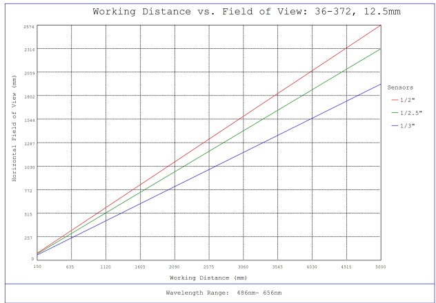
#36-372, 12.5mm FL f/2.5, Rugged Blue Series M12 Lens, Working Distance versus Field of View Plot
