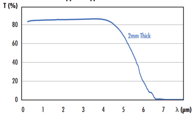
Sapphire Typical Transmission
