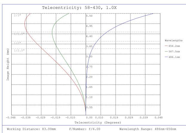
#58-430, 1.0X SilverTL™ Telecentric Lens, Telecentricity Plot
