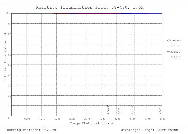
#58-430, 1.0X SilverTL™ Telecentric Lens, Relative Illumination Plot
