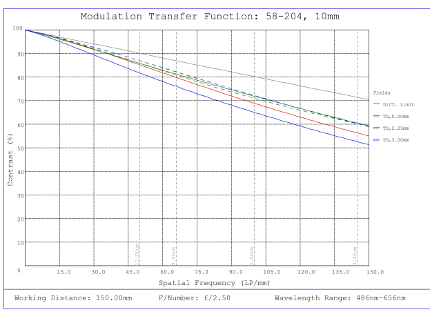
#58-204, 10mm FL f/2.5, Blue Series M12 Lens, Modulated Transfer Function (MTF) Plot, 150mm Working Distance, f2.5
