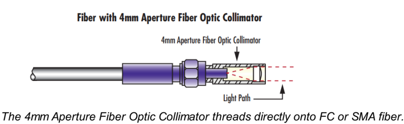
The 4mm Aperture Fiber Optic Collimator threads directly onto FC or SMA fiber.
