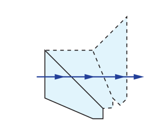
Half-Penta Prism Tunnel Diagram
