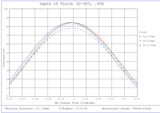
#62-903, 0.9X, 28.7mm M42 x 1.0 (6.56mm) PlatinumTL™ Telecentric Lens, Depth of Field Plot, 111mm Working Distance, f10
