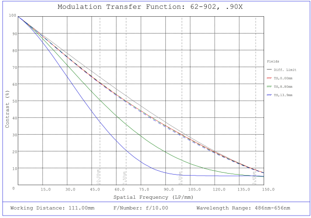
#62-902, 0.9X, 28.7mm F-Mount PlatinumTL™ Telecentric Lens, Modulated Transfer Function (MTF) Plot, 111mm Working Distance, f10
