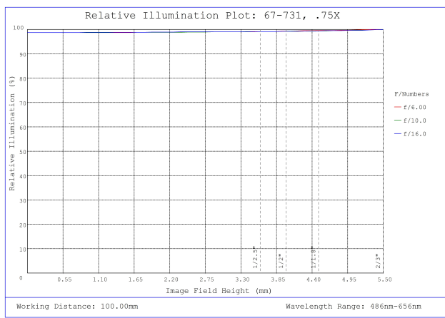
#67-731, 0.75X SilverTL™ Telecentric Lens, Relative Illumination Plot
