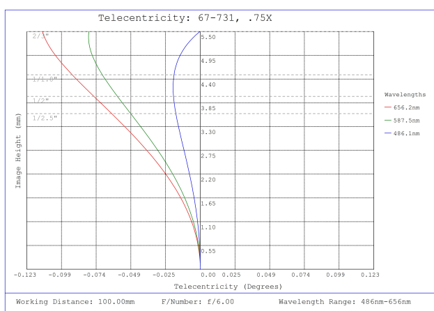
#67-731, 0.75X SilverTL™ Telecentric Lens, Telecentricity Plot
