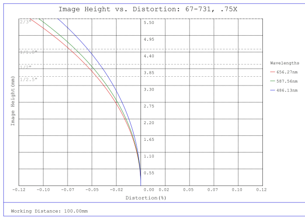
#67-731, 0.75X SilverTL™ Telecentric Lens, Distortion Plot
