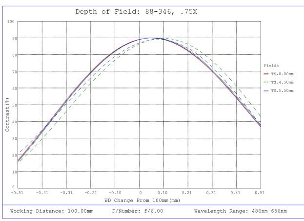
#88-346, 0.75X In-Line Illumination SilverTL™ Telecentric Lens, Depth of Field Plot, 100mm Working Distance, f6
