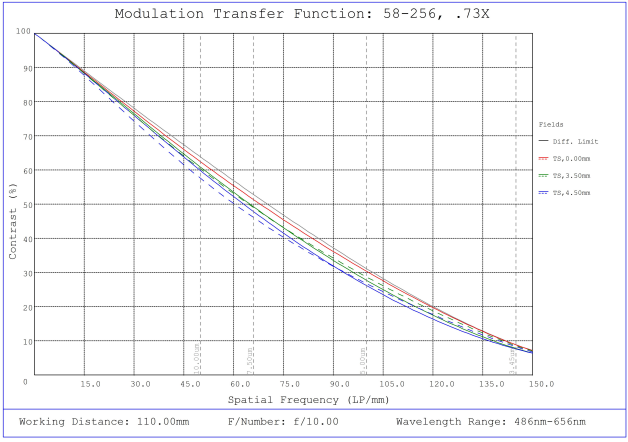
#58-256, 0.73X ½" GoldTL™ Telecentric Lens, Modulated Transfer Function (MTF) Plot, 110mm Working Distance, f10
