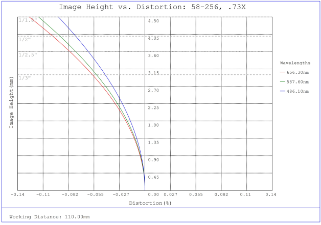
#58-256, 0.73X 1/2" GoldTL™ Telecentric Lens, Distortion Plot
