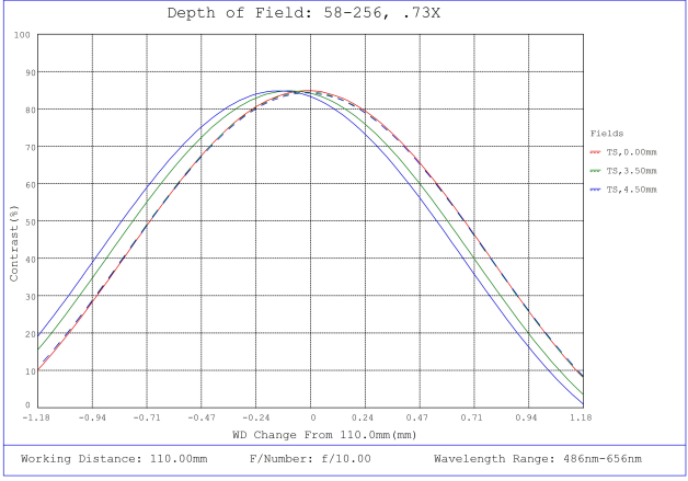
#58-256, 0.73X ½" GoldTL™ Telecentric Lens, Depth of Field Plot, 110mm Working Distance, f10
