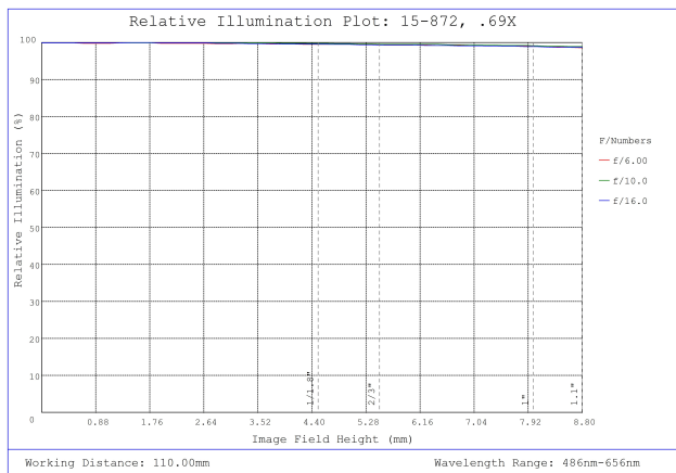
#15-872, 0.69X Cobalt TL Telecentric Lens, Relative Illumination Plot
